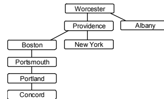
depth-first spanning tree:
