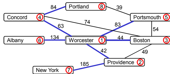
breadth-first spanning tree:
